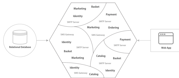
Figure 4: A Traditional Monolithic Legacy Software System (Case Study) (Silva et al., 2019)
