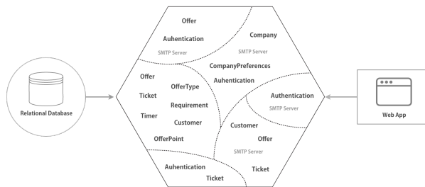
Figure 1: Entities and Associated Features Scattered and Tangled in ePromo (Silva et al., 2019)
