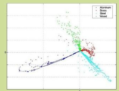
Fig. 3 – Principal components of impacts on rods.
