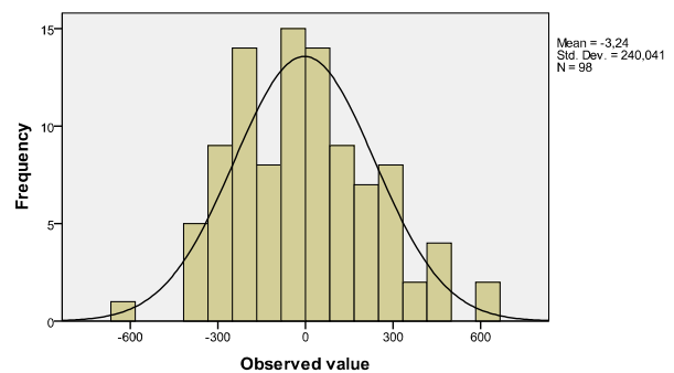
Figure 9. STC series
