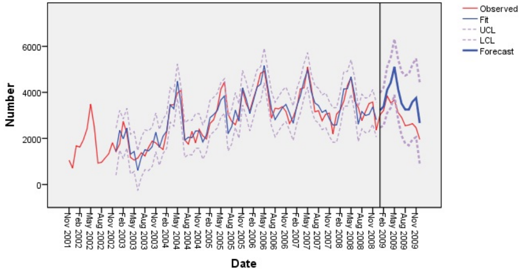
Figure 14. ARIMA(1,1,0), (1,1,0)
