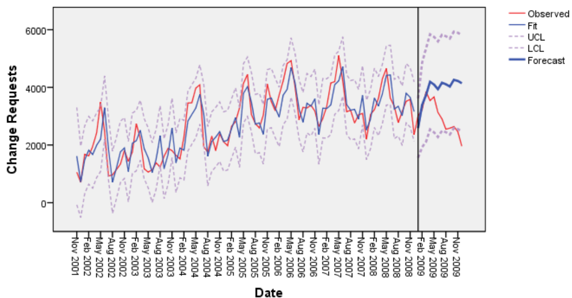
Figure 15. ARIMA(5,0,5)(0,0,0)
