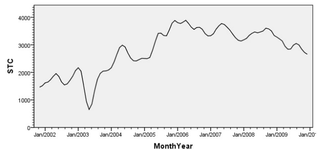
Figure 8. STC series
