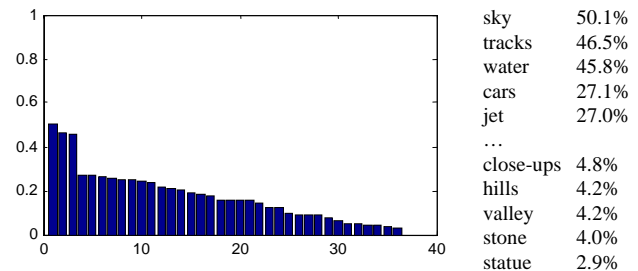
Figure 2. Average precision by concept.
