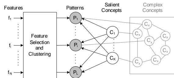
Figure 1. The incremental information extraction framework.
