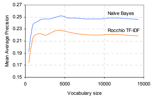
Figure 1 – Retrieval accuracy for 1 keyword.
