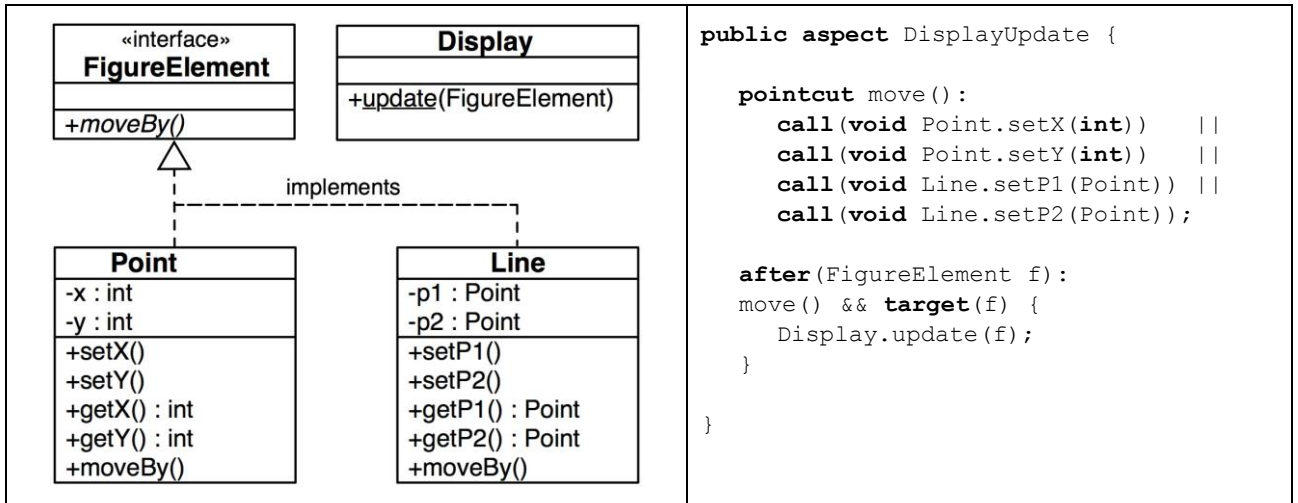
Figure 3: Illustrating example of the pointcut and advice mechanisms of AspectJ.
